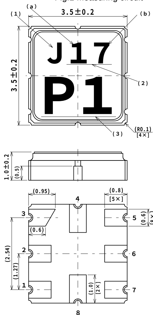
Fig.2 Package dimensions (in mm)
